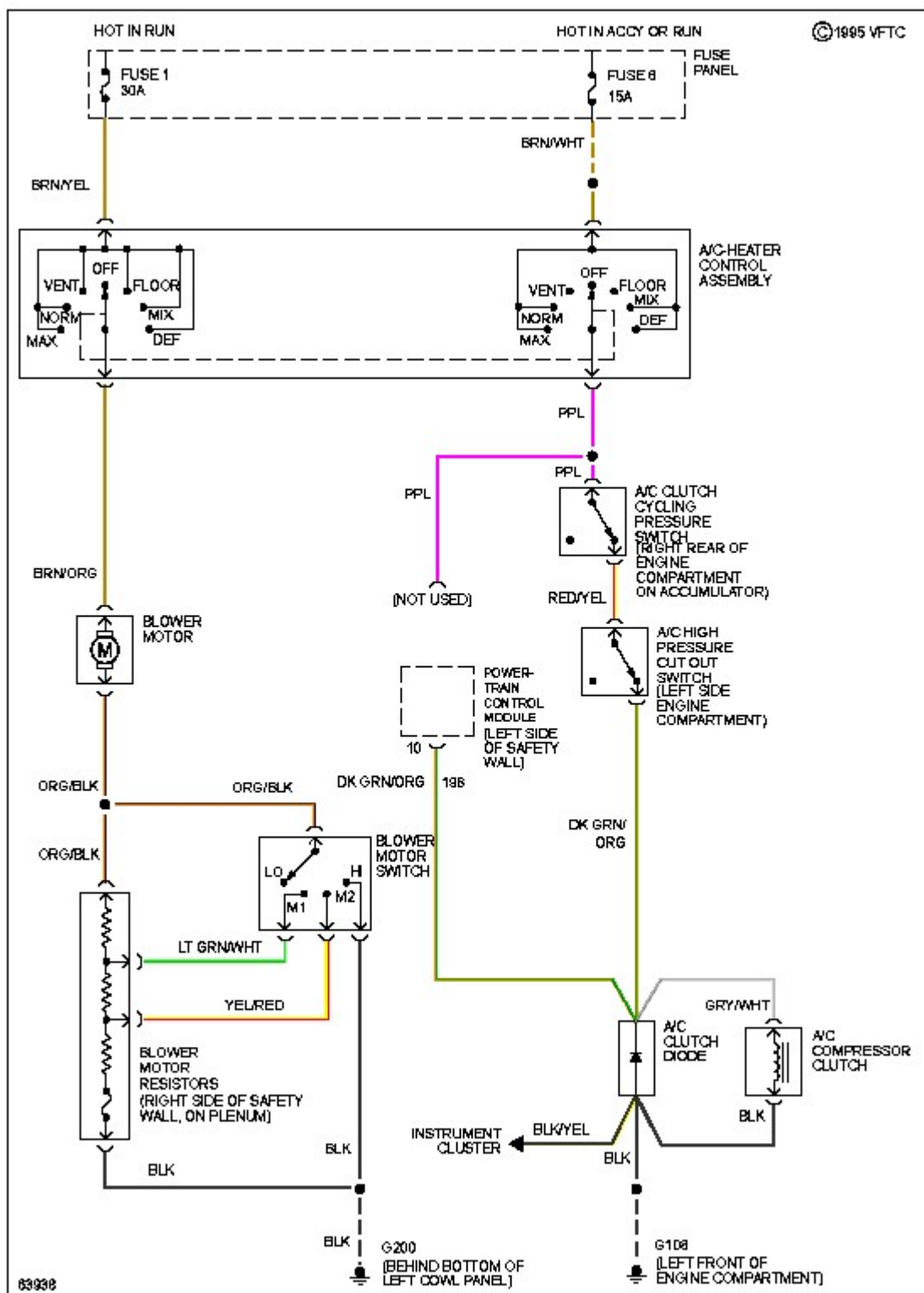
Fig. 1: A/C Circuit
