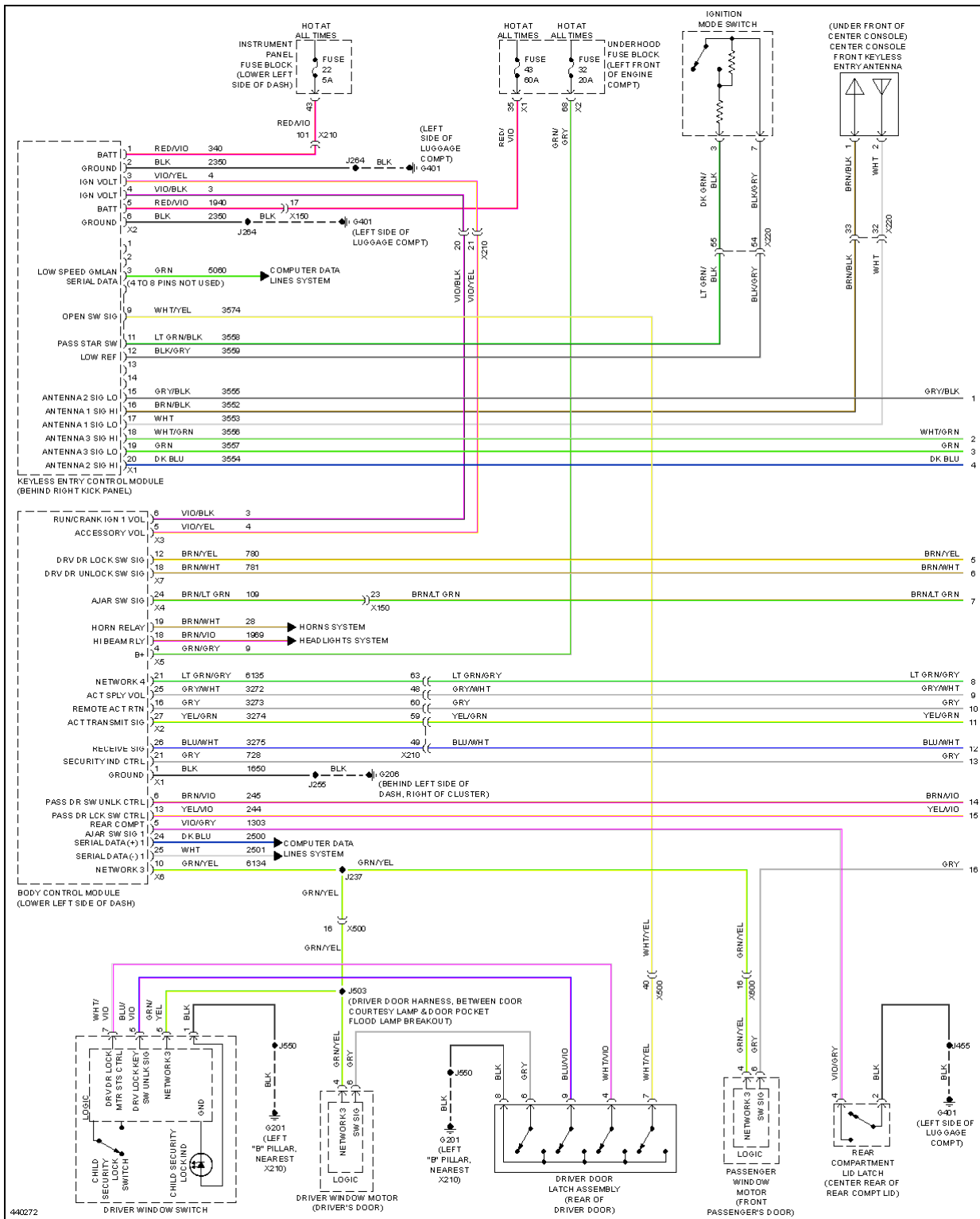
Fig. 7: Forced Entry Circuit, W/ Passive Keyless Entry (1 of 3)
