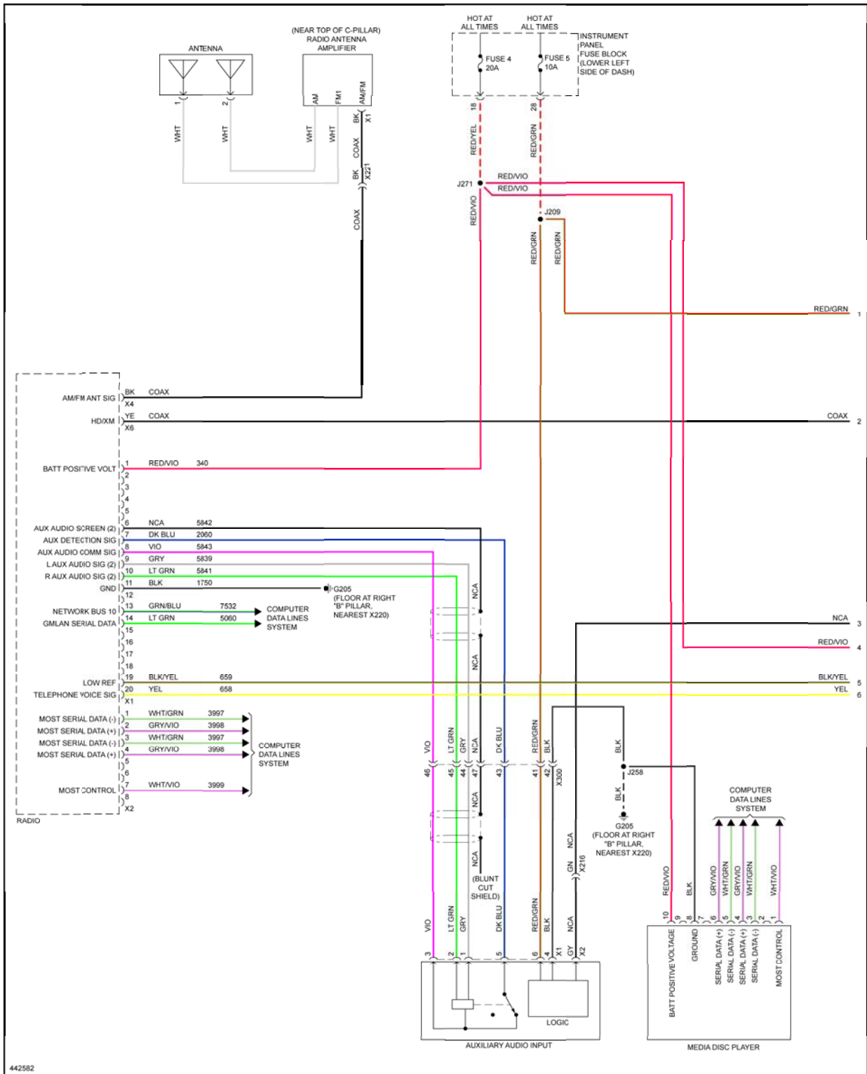
Fig. 106: Radio Circuit, W/O Amplifier (1 of 4)
